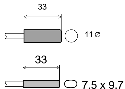
Normfühler 31..
